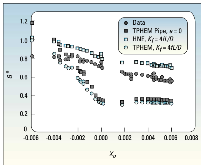
Figure 5. Sozzi and Sutherland Nozzle No. 3 data, L = 0.185 in.
